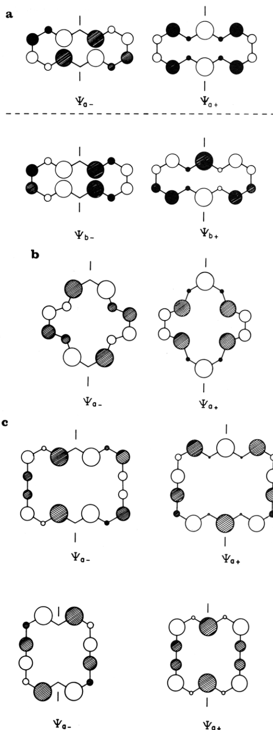
Figure 3. Schematic representation of the frontier orbitals of annulenes. (The areas of the circles are proportional to the squares of the LCAO coefficients, dotted and blank circles symbolize different signs.) (a) [14]Annulene with anthracene perimeter. (b) [14]Annulene with pyrene perimeter (LUMO's only). (c) Bisdehydro[18]annulene and bisdehydro[14]annulene (LUMO's only).
